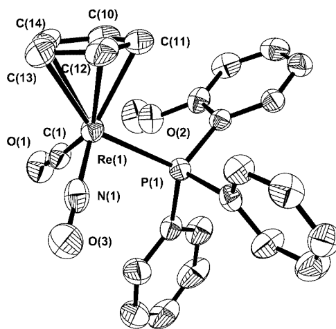
Figure 2. Structure of the cation of [CpRe(CO)(NO){PPh 2 (2-C 6 H 4 OMe)}]BF 4 ( 3a ), hydrogen atoms omitted for clarity. Space group P2 1 / c ; selected distances [pm] and angles (°) (standard deviations in parentheses): Re(1)–C(10) 228.2(7), Re(1)–C(11) 229.7(6), Re(1)–C(12) 231.8(6), Re(1)–C(13) 229.9(6), Re(1)–C(14) 229.9(7), Re(1)–C(1) 191.6(6), Re(1)–N(1) 180.1(6), Re(1)–P(1) 239.26(14); Re(1)–C(1)–O(1) 175.1(6), Re(1)–N(1)–O(2) 178.8(5), N(1)–Re(1)–C(1) 97.2(3), P(1)–Re(1)–N(1) 91.37(17), P(1)–Re(1)–C(1) 88.32(18).
