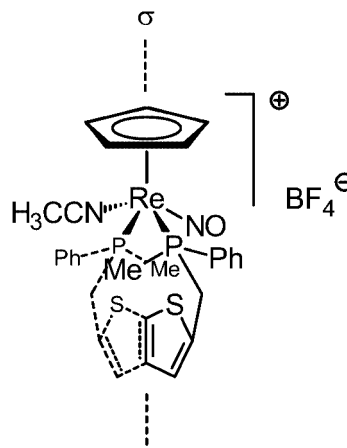
Figure 8. Disorder in the structure of unlike - 6e ; the phosphane ligand is reflected along an imaginary mirror plane which contains the Cp centre, the rhenium atom and two carbon atoms of the thiophene moiety giving rise to the like diastereoisomer
