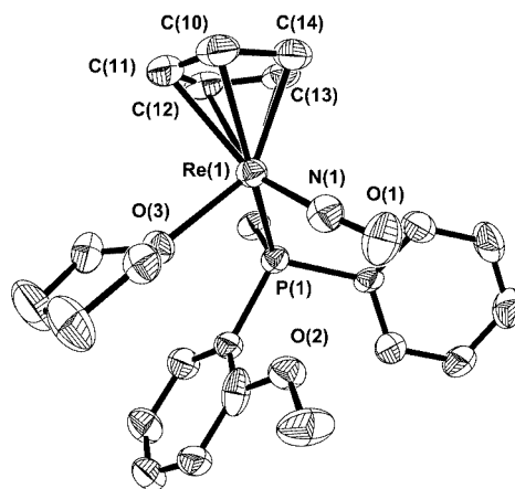
Figure 9. Structure of the cation of (S_{Re}, S_P/R_{Re}, R_P) -[CpRe(NO){P(Ph)(Me)(2-C 6 H 4 OMe)}(THF)]BF 4 ( 7d ), hydrogen atoms omitted for clarity. Space group P2_1/c ; selected distances [pm] and angles ( ^\circ ) (standard deviations in parentheses): Re(1)–C(10) 228.9(8), Re(1)–C(11) 235.0(8), Re(1)–C(12) 230.6(8), Re(1)–C(13) 220.8(7), Re(1)–C(14) 217.7(8), Re(1)–N(1) 174.9(7), Re(1)–O(3) 214.6(5), Re(1)–P(1) 238.64(18); Re(1)–N(1)–O(1) 176.0(7), N(1)–Re(1)–O(3) 96.9(3), P(1)–Re(1)–N(1) 90.8(2), P(1)–Re(1)–O(3) 87.60(14)
