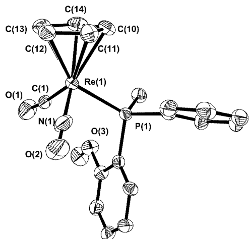
Figure 4. Structure of the cation of [\text{CpRe}(\text{CO})(\text{NO})\{\text{P}(\text{Ph})(\text{Me})(2-\text{C}_6\text{H}_4\text{OMe})\}]\text{AlF}_4 ( 3d-AlF 4 ), hydrogen atoms omitted for clarity. Space group P2_1/n ; selected distances [pm] and angles ( ^\circ ) (standard deviations in parentheses): \text{Re}(1)-\text{C}(10) 231.7(7), \text{Re}(1)-\text{C}(11) 229.3(7), \text{Re}(1)-\text{C}(12) 227.7(7), \text{Re}(1)-\text{C}(13) 229.4(7), \text{Re}(1)-\text{C}(14) 227.5(7), \text{Re}(1)-\text{C}(1) 186.2(6), \text{Re}(1)-\text{N}(1) 183.3(7), \text{Re}(1)-\text{P}(1) 239.65(17), \text{Re}(1)-\text{C}(1)-\text{O}(1) 173.1(7), \text{Re}(1)-\text{N}(1)-\text{O}(2) 176.3(8), \text{N}(1)-\text{Re}(1)-\text{C}(1) 95.8(3), \text{P}(1)-\text{Re}(1)-\text{N}(1) 89.6(2), \text{P}(1)-\text{Re}(1)-\text{C}(1) 91.1(2)
