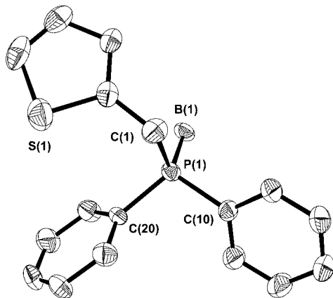
Figure 1. Molecular structure of PPh 2 (CH 2 C 4 H 3 S)·BH 3 ( 1b ·BH 3 ), hydrogen atoms omitted for clarity. Space group Pna 2 1 ; selected distances [pm] and angles (°) (standard deviations in parentheses): P(1)–B(1) 190.4(4), P(1)–C(1) 182.9(3), P(1)–C(10) 181.2(3), P(1)–C(20) 180.6(3); C(1)–P(1)–B(1) 111.98(19), C(10)–P(1)–B(1) 110.52(17), C(20)–P(1)–B(1) 117.02(17), C(1)–P(1)–C(10) 105.82(16), C(1)–P(1)–C(20) 104.13(17), C(10)–P(1)–C(20) 106.58(15).
