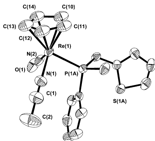
Figure 7. Structure of the cation of (R_{Re}, S_P/S_{Re}, R_P) -[CpRe(NO){P(Ph)(Me)(CH 2 C 4 H 3 S)}(NCCH 3 )]BF 4 ( 6e ), hydrogen atoms omitted for clarity. Space group P2_1/c ; selected distances [pm] and angles ( ^\circ ) (standard deviations in parentheses): Re(1)–C(10) 222.3(8), Re(1)–C(11) 228.3(8), Re(1)–C(12) 231.9(8), Re(1)–C(13) 226.9(7), Re(1)–C(14) 221.6(8), Re(1)–N(1) 205.5(6), Re(1)–N(2) 176.0(6), Re(1)–P(1A) 236.3(2); Re(1)–N(2)–O(1) 178.9(5), Re(1)–N(1)–C(1) 176.9(6), N(1)–C(1)–C(2) 178.6(8), N(1)–Re(1)–N(2) 96.9(2), P(1A)–Re(1)–N(1) 85.03(17), P(1A)–Re(1)–N(2) 92.86(18)
