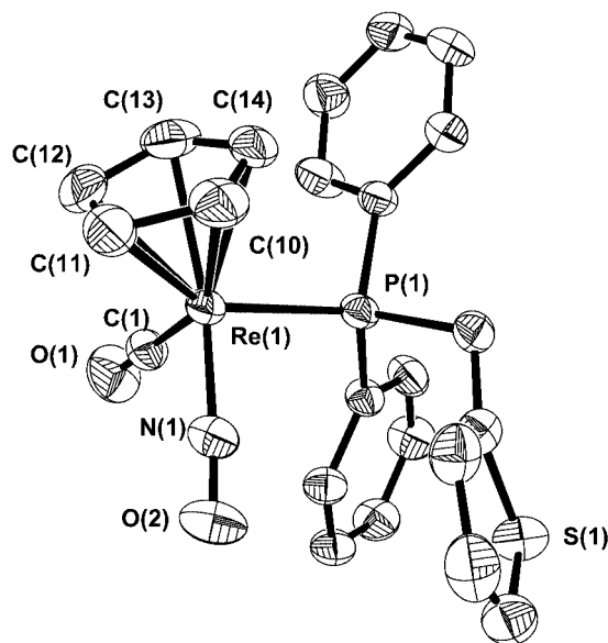
Figure 3. Structure of the cation of [\text{CpRe}(\text{CO})(\text{NO})\{\text{PPh}_2-(\text{CH}_2\text{C}_4\text{H}_3\text{S})\}]\text{BF}_4 ( 3b ), hydrogen atoms omitted for clarity. Space group P1 ; selected distances [pm] and angles ( ^\circ ) (standard deviations in parentheses): \text{Re}(1)-\text{C}(10) 231.4(5), \text{Re}(1)-\text{C}(11) 227.8(6), \text{Re}(1)-\text{C}(12) 227.1(6), \text{Re}(1)-\text{C}(13) 228.1(6), \text{Re}(1)-\text{C}(14) 231.5(5), \text{Re}(1)-\text{C}(1) 188.4(5), \text{Re}(1)-\text{N}(1) 182.6(4), \text{Re}(1)-\text{P}(1) 239.05(12), \text{Re}(1)-\text{C}(1)-\text{O}(1) 179.7(5), \text{Re}(1)-\text{N}(1)-\text{O}(2) 175.7(4), \text{N}(1)-\text{Re}(1)-\text{C}(1) 92.4(2), \text{P}(1)-\text{Re}(1)-\text{N}(1) 95.56(14), \text{P}(1)-\text{Re}(1)-\text{C}(1) 89.70(16)
