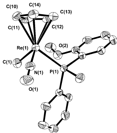
Figure 5. Molecular structure of ( R_{\text{Re}}, S_{\text{P}}, S_{\text{Re}}, R_{\text{P}} ) [\text{CpRe}(\text{NO})\{\text{P}(\text{Ph})(\text{Me})(2\text{-C}_6\text{H}_4\text{OMe})\}\{\text{CH}_3\}] ( 4d ), hydrogen atoms omitted for clarity. Space group P1 ; selected distances [pm] and angles ( ^\circ ) (standard deviations in parentheses): \text{Re}(1)\text{--C}(10) 228.4(4), \text{Re}(1)\text{--C}(11) 234.0(4), \text{Re}(1)\text{--C}(12) 233.6(4), \text{Re}(1)\text{--C}(13) 225.7(4), \text{Re}(1)\text{--C}(14) 222.8(4), \text{Re}(1)\text{--C}(1) 214.1(4), \text{Re}(1)\text{--N}(1) 175.6(3), \text{Re}(1)\text{--P}(1) 234.30(9), \text{Re}(1)\text{--N}(1)\text{--O}(1) 177.9(3), \text{N}(1)\text{--Re}(1)\text{--C}(1) 95.55(18), \text{P}(1)\text{--Re}(1)\text{--N}(1) 88.89(11), \text{P}(1)\text{--Re}(1)\text{--C}(1) 90.24(12).
