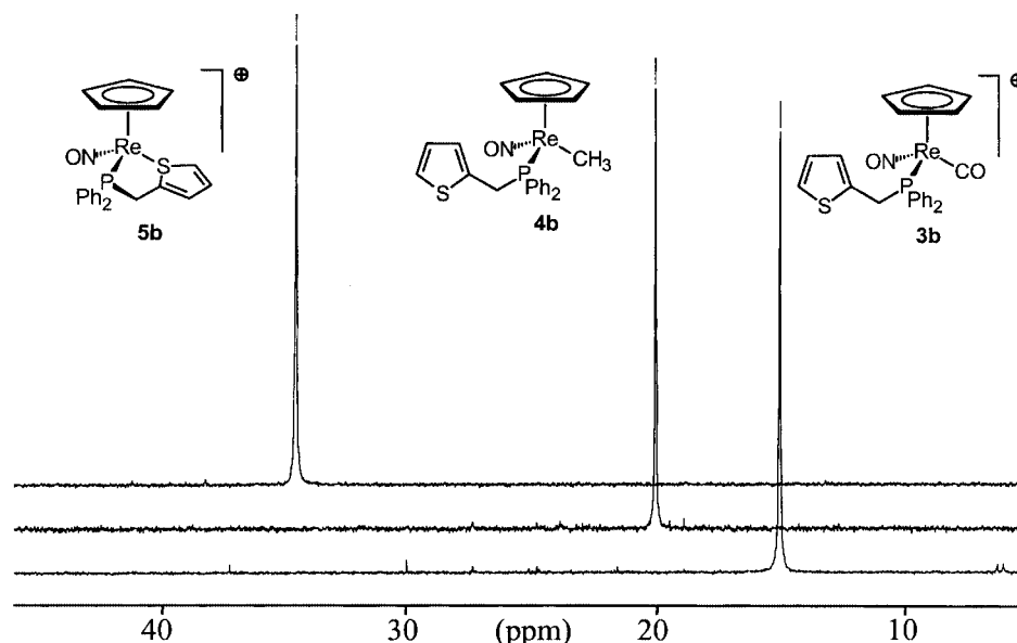
Figure 6. ^{31}\text{P} NMR spectra of the complexes [\text{CpRe}(\text{NO})\{\text{PPh}_2(\text{CH}_2\text{C}_4\text{H}_3\text{S})\}(\text{X})]\text{Y} ; \text{X} = \text{CO} , \text{Y} = \text{BF}_4 3b , \text{X} = \text{CH}_3 , \text{Y} = - 4b , \text{X} = - , \text{Y} = \text{BF}_4 5b .
